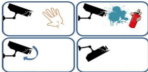
Tampering Detection
