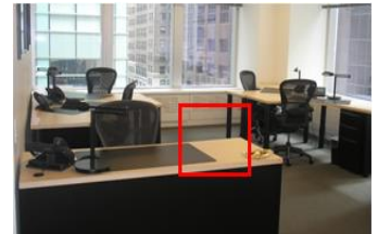
Missing Object
