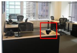
Unattended Object
