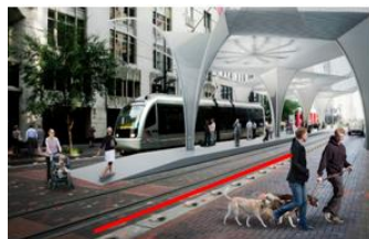
Line Crossing
